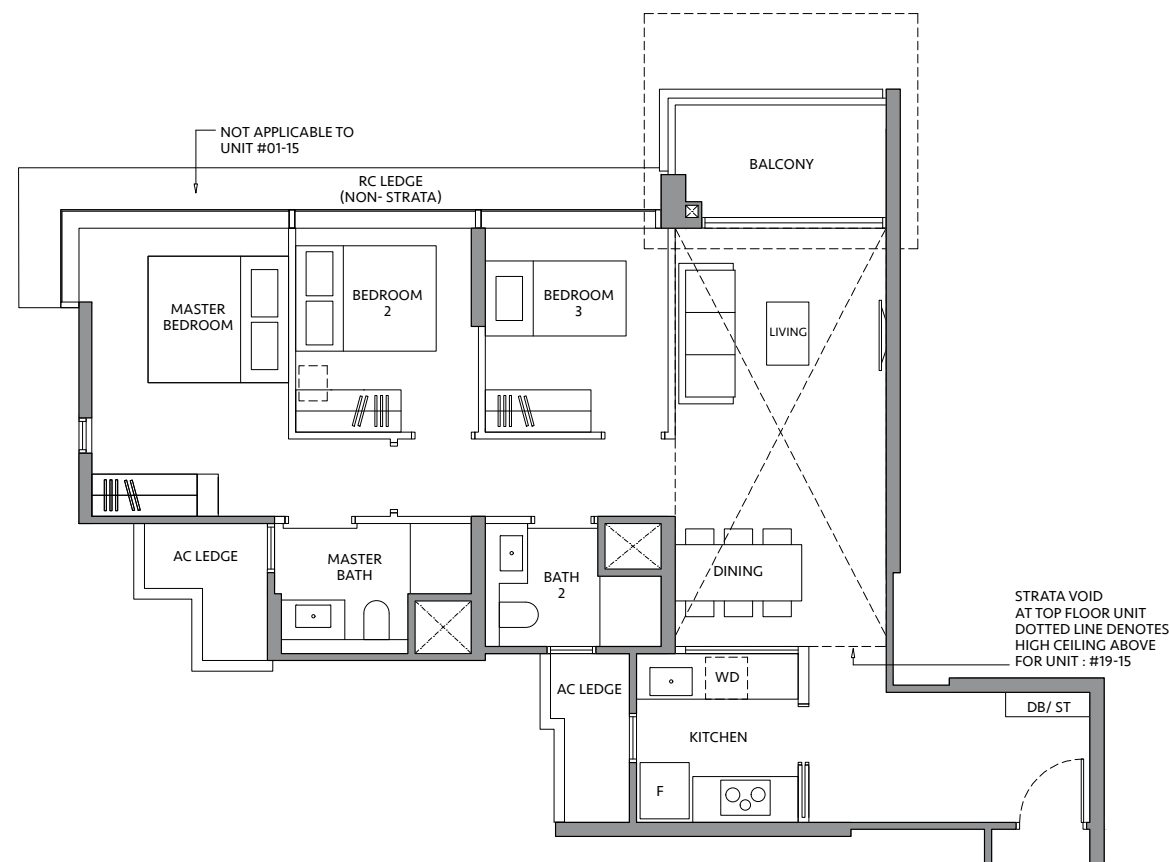
APPLICABLE TO UNIT #01-15
