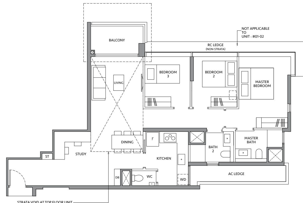
STRATA VOID AT TOP FLOOR UNIT DOTTED LINE DENOTES HIGH CEILING ABOVE FOR UNIT: #19-02
